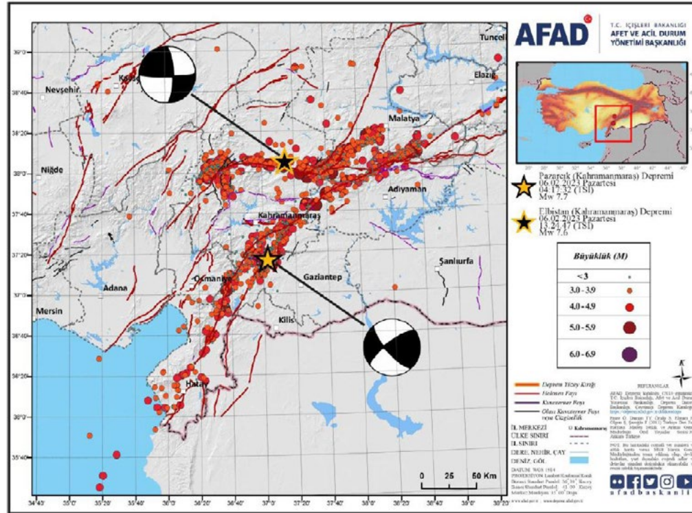
Figure 1: 06 February 2023 Pazarcık (Kahramanmaraş) Mw 7.7 and Elbistan (Kahramanmaraş) Mw 7.6 earthquakes and aftershock activity.
