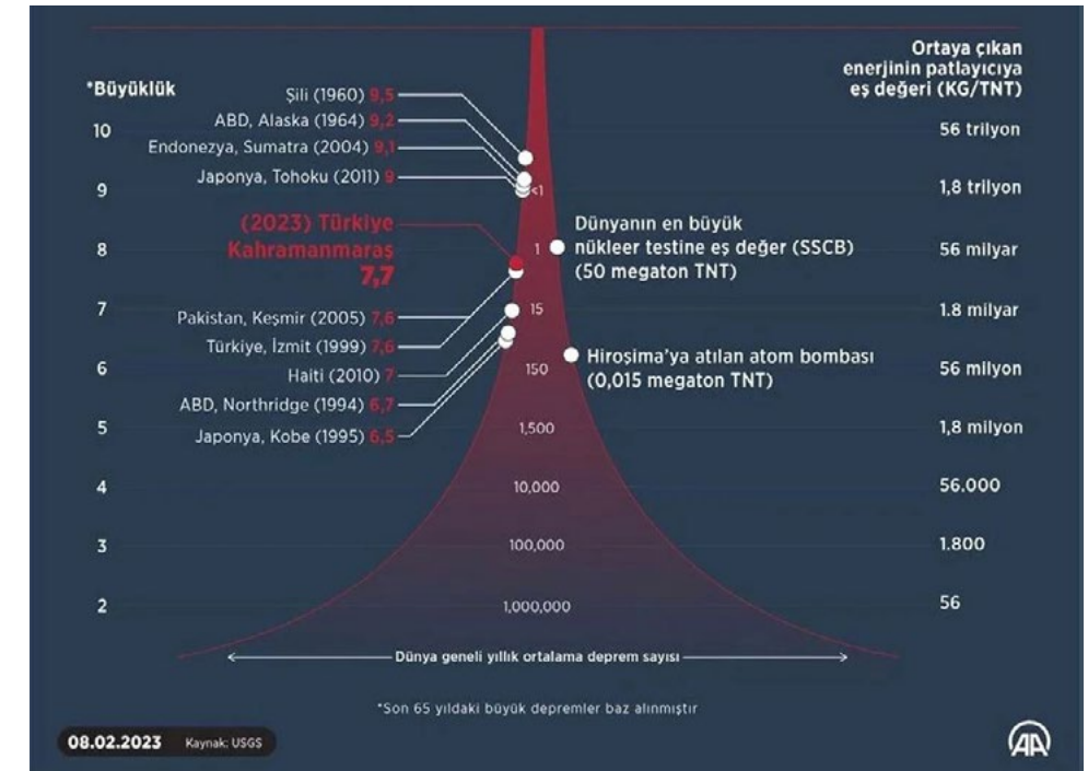
Figure 2: Intensity and magnitude of earthquakes.
